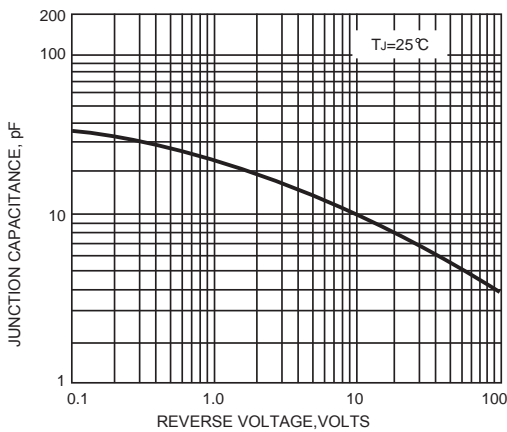
FIG. 5-TYPICAL JUNCTION CAPACITANCE
